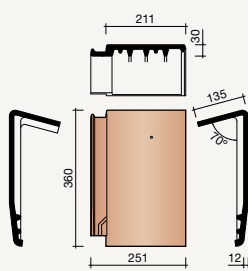
8500 Chaperonpan
