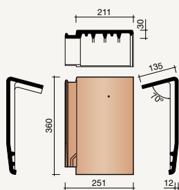
8500 Chaperonpan
