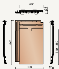
0000 Actua 10 EB dakpan
